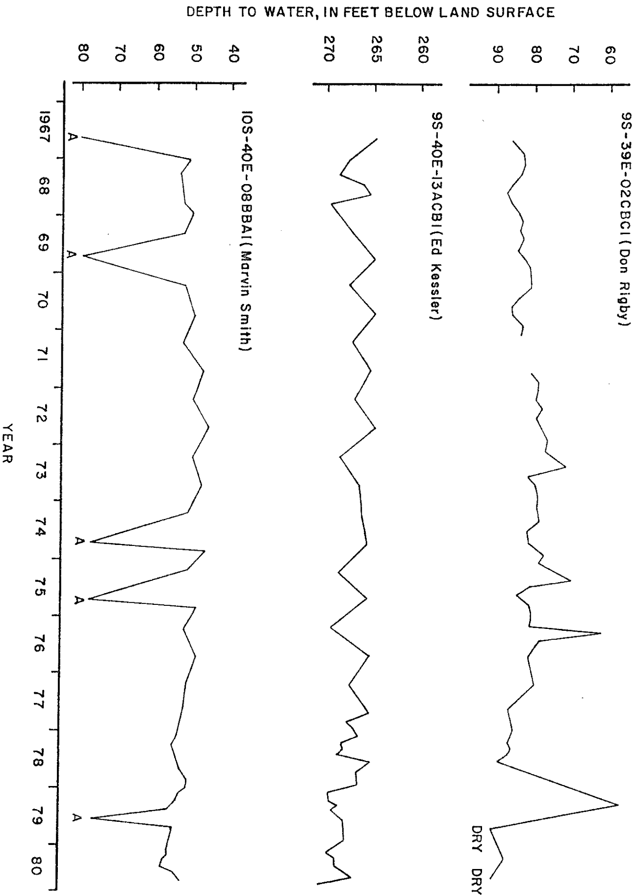
Figure 9. Hydrographs showing long term ground water level fluctuations.
