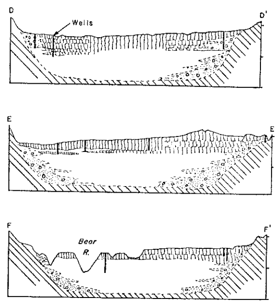
Figure 2. Geologic map of Thatcher Basin and geologic cross sections (Bright, 1963).
