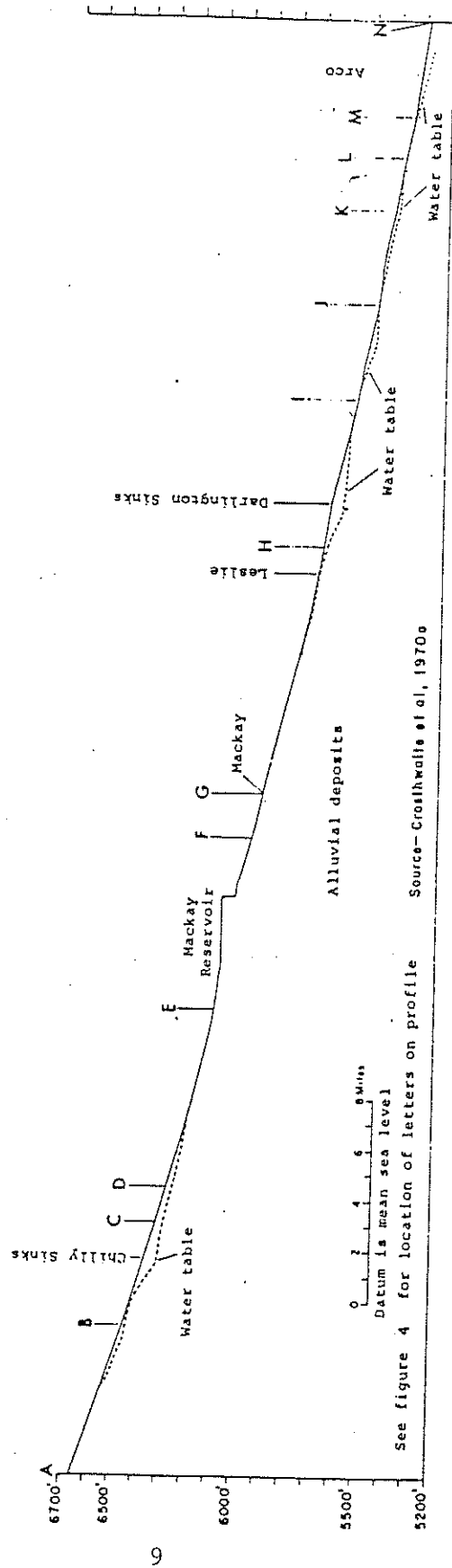
FIGURE 3----- Profile of Big Lost River showing the position of the water table.
