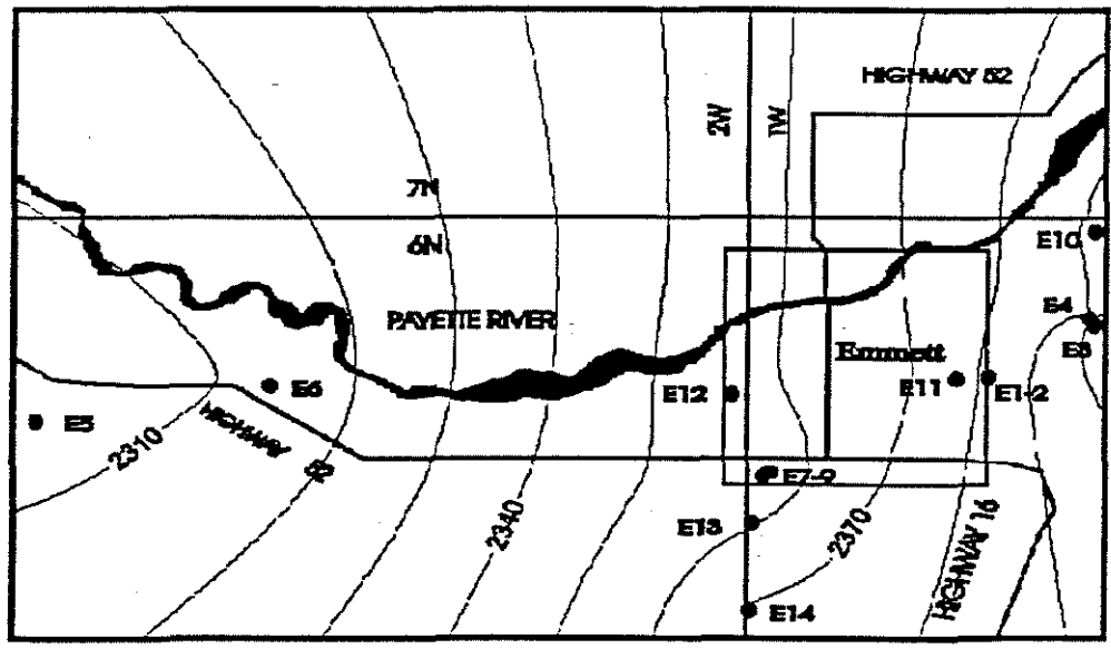
Figure 2. Location and Ground Water Contours of Wells
