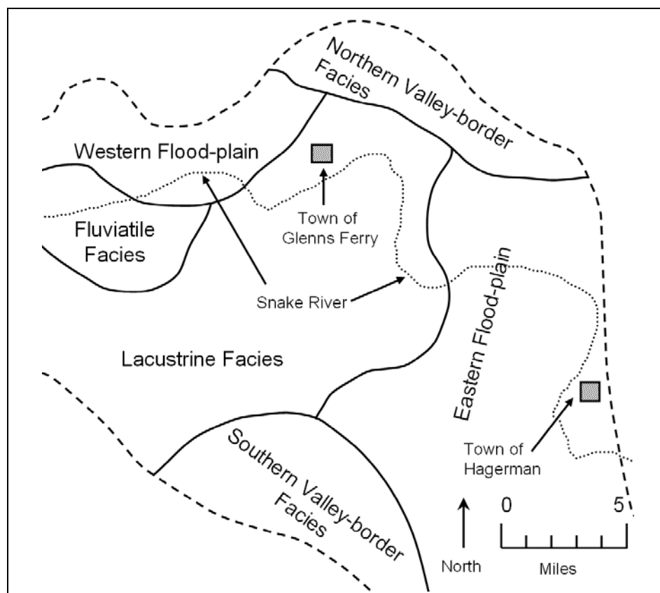
Figure 8. Distribution Glens Ferry Formation sedimentary facies in the Glens Ferry/Hagerman area (after Malde, 1972b).
