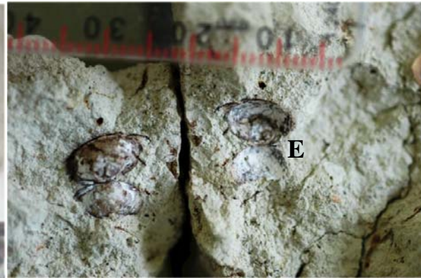
Figure 5. Fresh exposure of GFF (A) at Vader Grade road cut (B) and fossil willow leaves (C&D) and a bivalve (E). Note the darker horizontal banding above and left of the pickup truck from groundwater flowing through the GFF but not from the overlying basalt at this location. The top panorama photo is looking west from Rangen area with the Vader Grade in the foreground and the Hagerman Fossil Beds in the distance.
