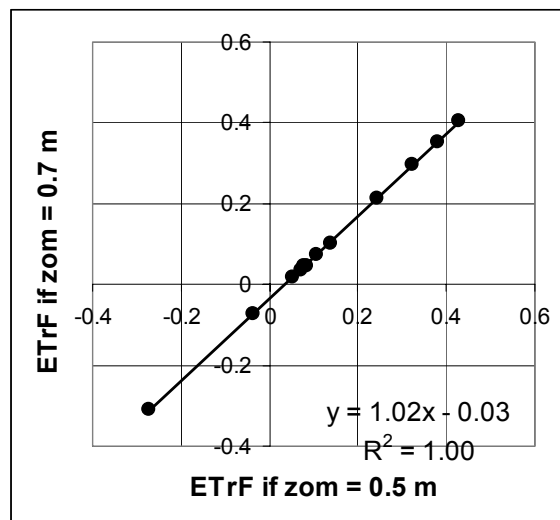
Figure 4.1.2.1.6-1. METRIC ET_rF for Twin Falls, Idaho, applying z_{om} = 0.5 m and applying z_{om} = 0.7 m for city areas on 8/14/2000.
