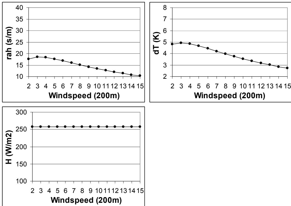
Figure 4.1.2.2.3-3. Sensitivity of r_{ah} , dT and H , for different windspeed levela at the selected hot pixel (dry agricultural bare field) in Path 40 Row 30, 7/5/2000.
